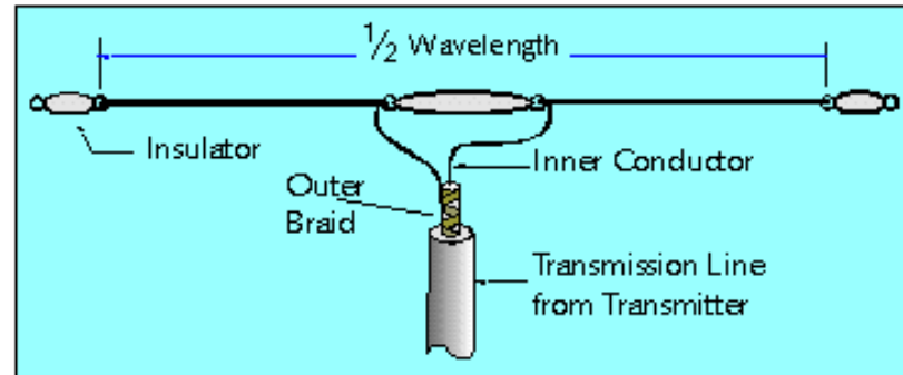
dipole antenna
